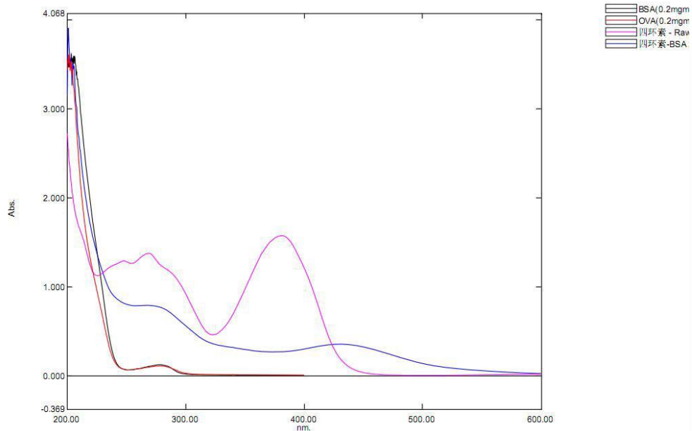
Figure 1. UV-spectrum
